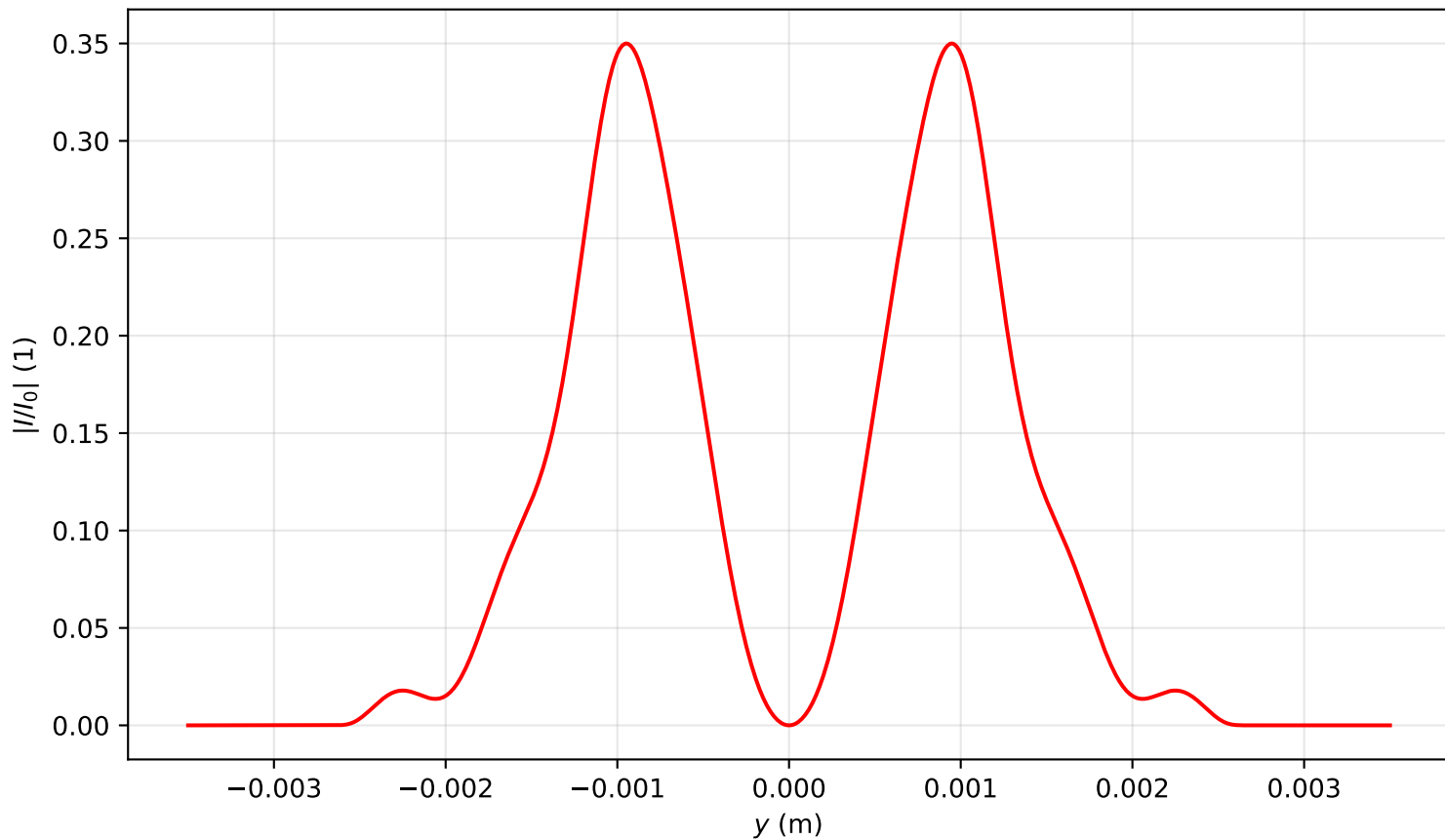
Intensity profile I(x=0, y, z=3.901)/I_0 , P_{in}=3.0P_{cr} , artificial time
